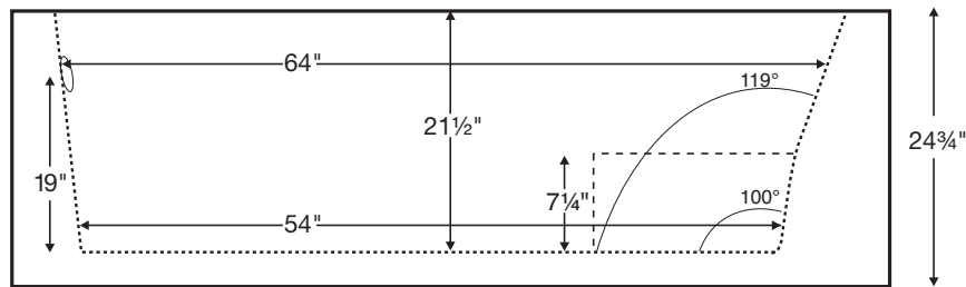
Optional Integral Armrests
